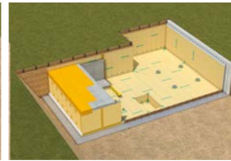
Sikaproof® / SikaBit S-515
